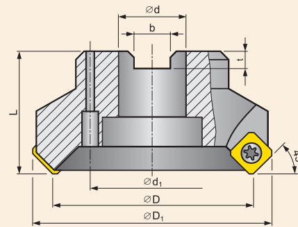
\varnothing 160 mm
