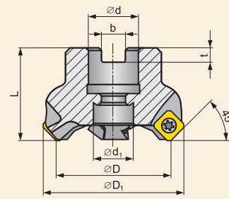
\varnothing 32 - 125 mm
