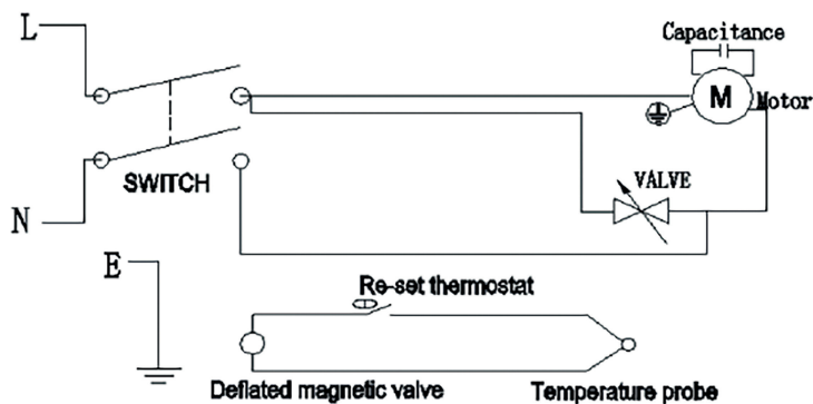
Fig. 4 Circuit diagram
